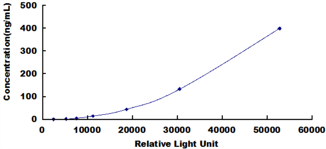
Typical Standard Curve for a1AT, Human CLIA.
